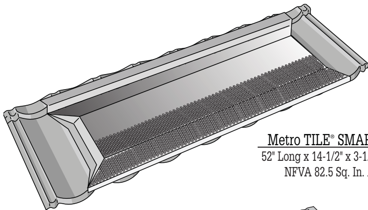
MetroROMAN® SMARTvent 52" Long x 14-1/2" x 3-1/2" High NFVA 82.5 Sq. In. Approx.
