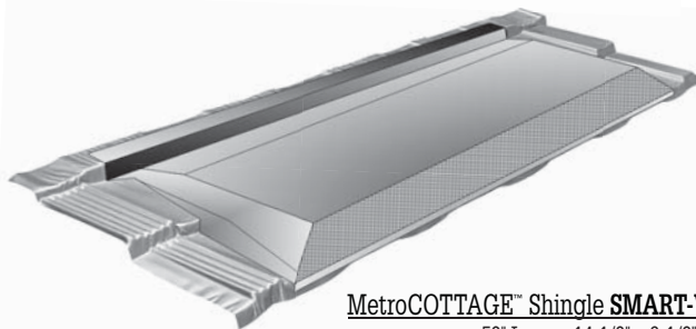
MetroSHAKE® SMART-Vent 52" Long x 14-1/2" x 3-1/2" High NFVA 82.5 Sq. In. Approx.
